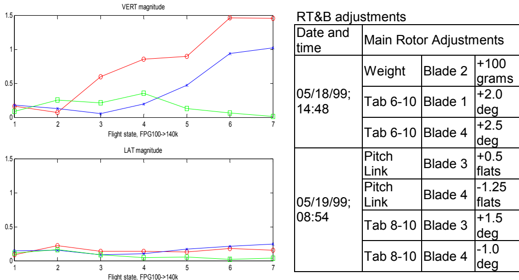
Figure 4 Preliminary tests at SCARNG on the AH-64 Apache tail number 460: Vibration magnitudes is shown for the first (o), second (x), and third ( ) flight in the series.
